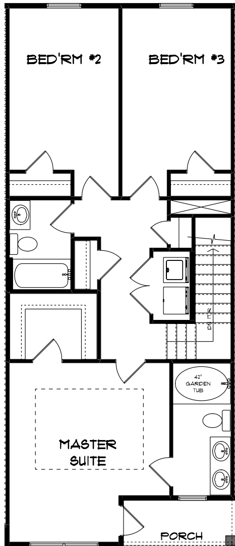
PLAN - B
