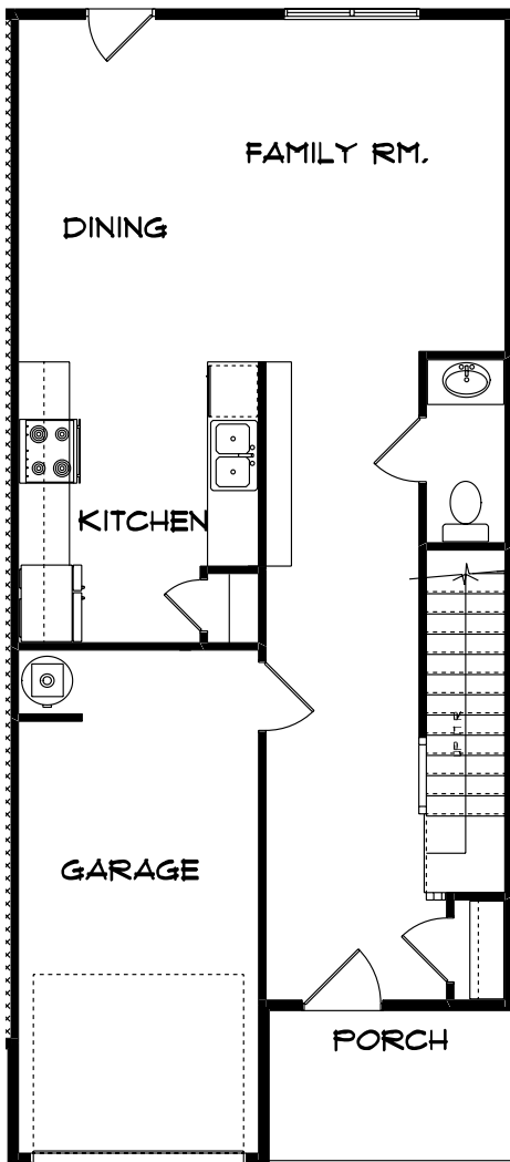
PLAN - C
